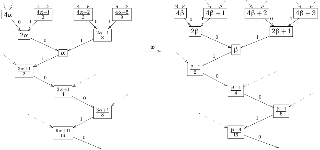
Figure 5: A divergent component in C(\mathbb{Z}_2) with an irrational number \alpha = 10110\dots (left), and the corresponding component in B(\mathbb{Z}_2) with the irrational number \Phi(\alpha) = \beta = 10010\dots (right). Note that the first five bits of \beta follow from \Phi_5(10110) = 10010 , or equivalently, \Phi_5(13) = 9 .
