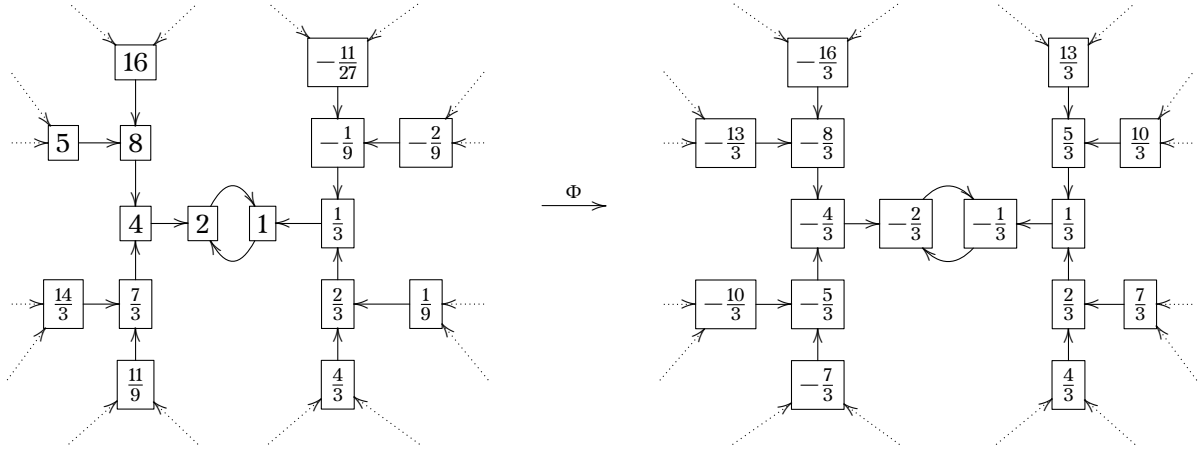
Figure 6: The components corresponding to the cycle (01), in C(\mathbb{Z}_2) (left) and in B(\mathbb{Z}_2) (right). The Collatz conjecture states that the component on the left contains all positive integers.
