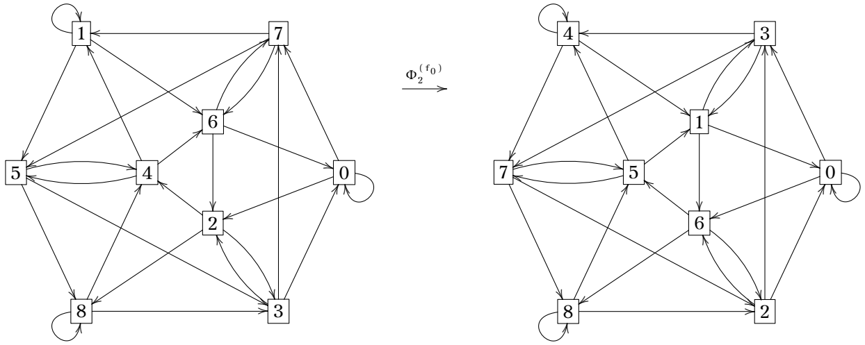
Figure 8: The ternary modular graph of dimension 2 corresponding to the function f_0 in (18) and the ternary De Bruijn graph of dimension 2, B(3,2) . The corresponding isomorphism \Phi_2^{(f_0)} of order 7 is given by the permutation \Phi_2^{(f_0)} \equiv (1, 4, 5, 7, 3, 2, 6) .
