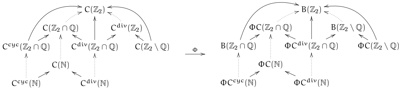
Figure 7: The structure inside C(\mathbb{Z}_2) (left) and the corresponding structure inside B(\mathbb{Z}_2) (right). Solid arrows pointing to the same larger graph imply that the large graph can be partitioned into these smaller graphs. Dotted lines correspond to graph inclusions.
